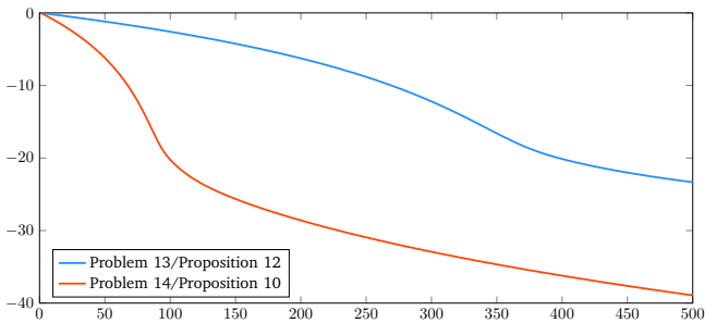
Fig. 3: Normalized error 20 \log_{10}(\|x_n - x_\infty\|/\|x_0 - x_\infty\|) (dB) versus iteration count in Experiment V-A.
